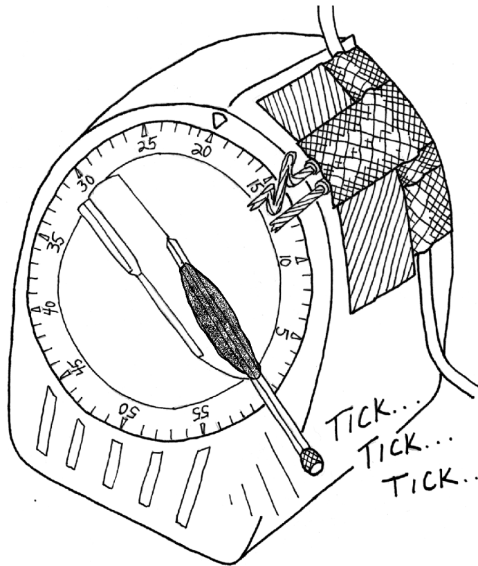
Figure G: Notice that the two wires curve away in opposite directions to allow the tape to grip them more firmly. Also notice that one of the ends has been kinked to guarantee that the two wires will contact each other.
